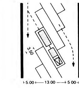
② 30° parking, truck with trailer
